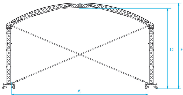
Front view - 6x4 m Arc
