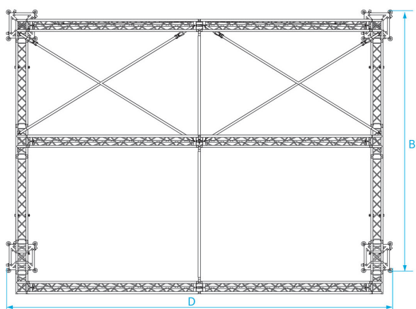
Top view - 6x4 m Arc
