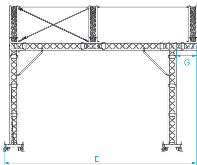
Side view - 6x4 m Arc
